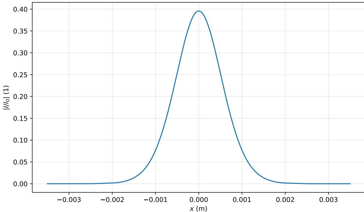
Intensity profile I(x, y = 0, z = 3.503m)/I_0 , P_{in}=0.4P_{cr} , artificial time
